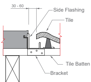
Side Detail
